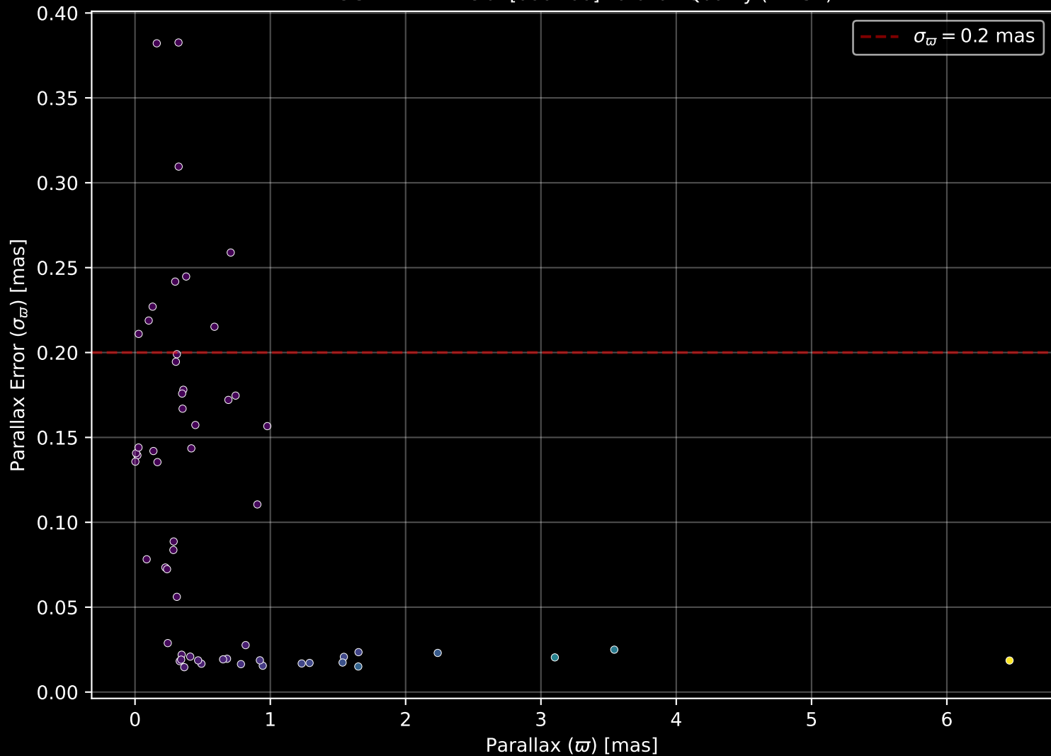
APOGEE DR17 Field: [006+00] Parallax Quality (n= 57)
