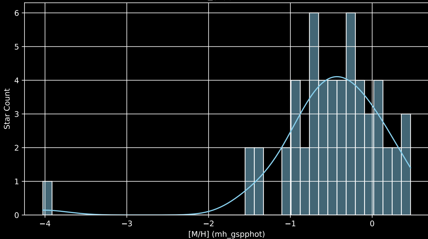
APOGEE DR17 Field: [006+00 [M/H] (mh_gspphot) (n= 55)
