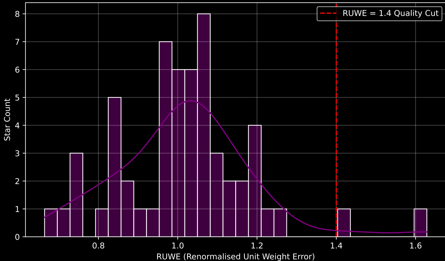
GAPOGEE DR17 Field [006+00] RUWE Distribution (n= 57)
