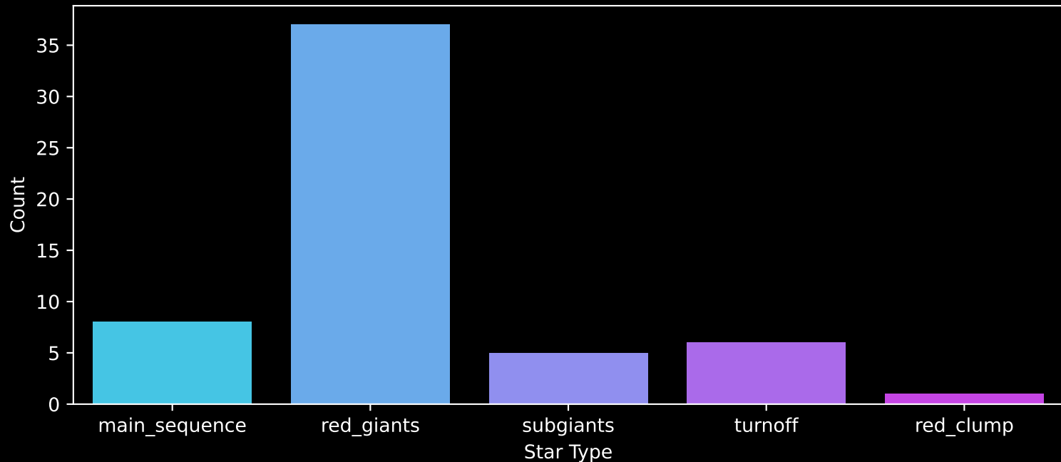
APOGEE DR17 Field: [006+00] Count plot of Star Type
