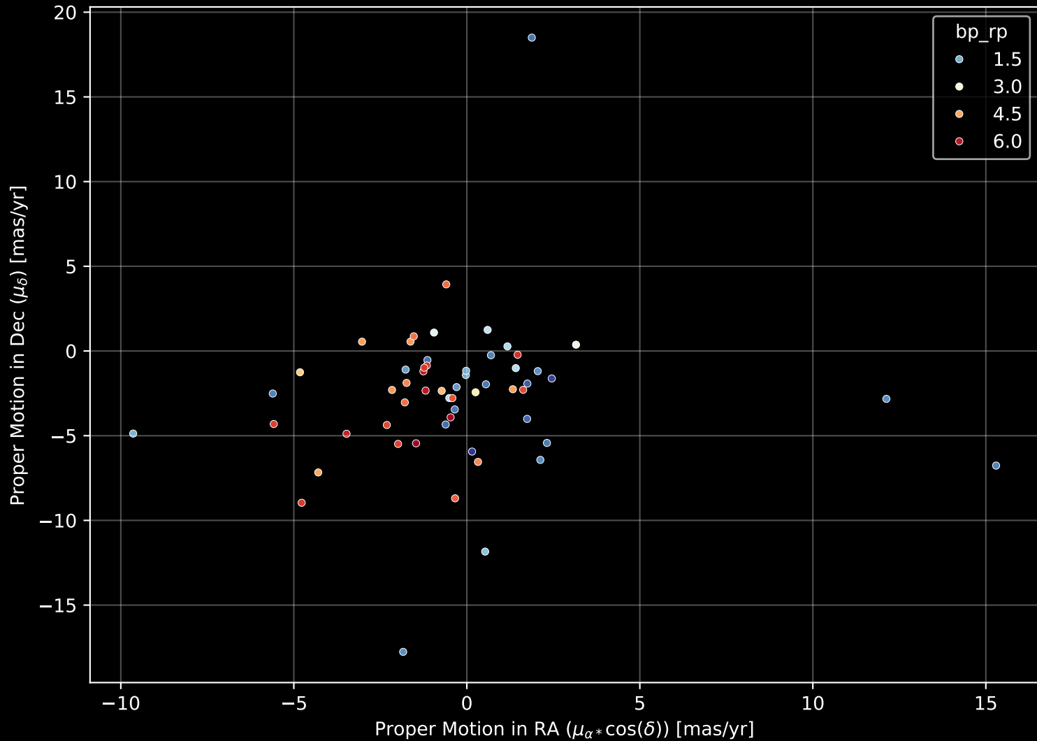
APOGEE DR17 Field: [006+00] Proper Motion Diagram (n= 57)
